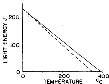
Fig 20 The relationship between light energy for ignition and temperature for lead azide (Ref 32). The solid line gives the experimental curve; the dotted line connects the value for the ignition energy at 20°C and the point on the temperature axis corresponding to the thermal ignition temperature
